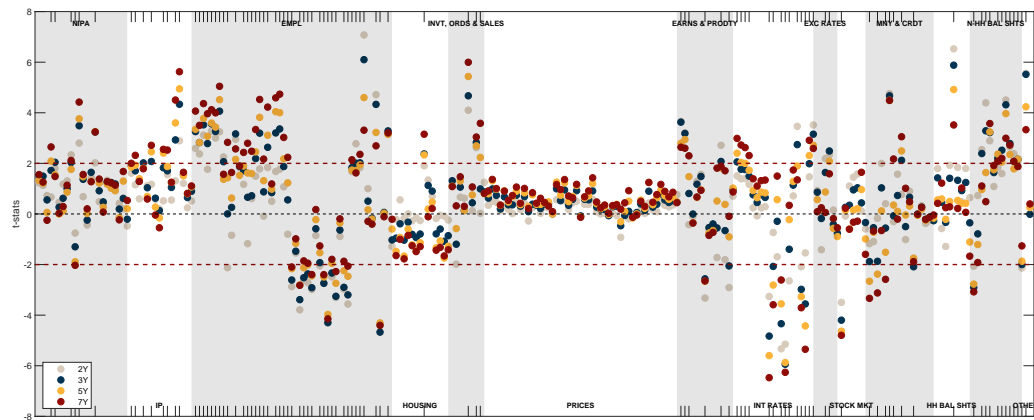
Figure 3.2: Markers indicate t -statistics from logit regressions of the EH state probabilities for maturities n = 2, 3, 5 and 7 on 248 individual macroeconomic variables from the FRED-QD database. Red dashed line indicates \pm 2 for reference. Shading indicates variable groups as defined in the appendix to McCracken and Ng (2016) (See table 3.3).
